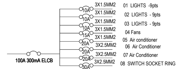
8WAYS TPN DISTRIBUTION BOARD THEATRE
