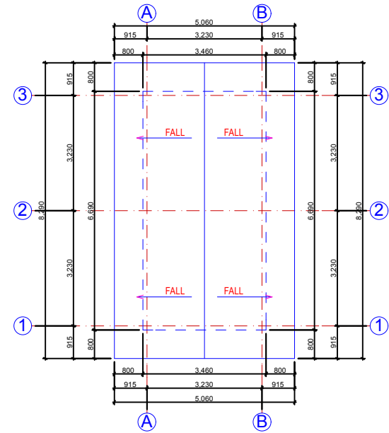
ROOF PLAN L[-]09
