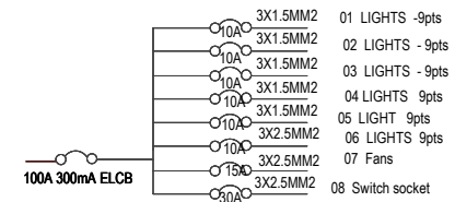
8WAYS TPN DISTRIBUTION BOARD MENTAL WARD
