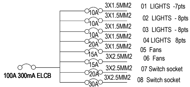
8WAYS TPN DISTRIBUTION BOARD MWH
