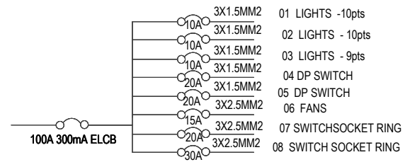
8WAYS TPN DISTRIBUTION BOARD LABORATORY
